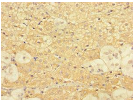
Immunohistochemistry of paraffin-embedded human adrenal gland tissue using PACO40374 at dilution of 1:100.
