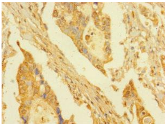
Immunohistochemistry of paraffin-embedded human pancreatic cancer using PACO40374 at dilution of 1:100.
