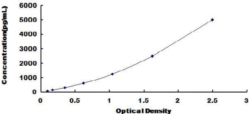
Typical Standard Curve for Human VNN1 ELISA.
